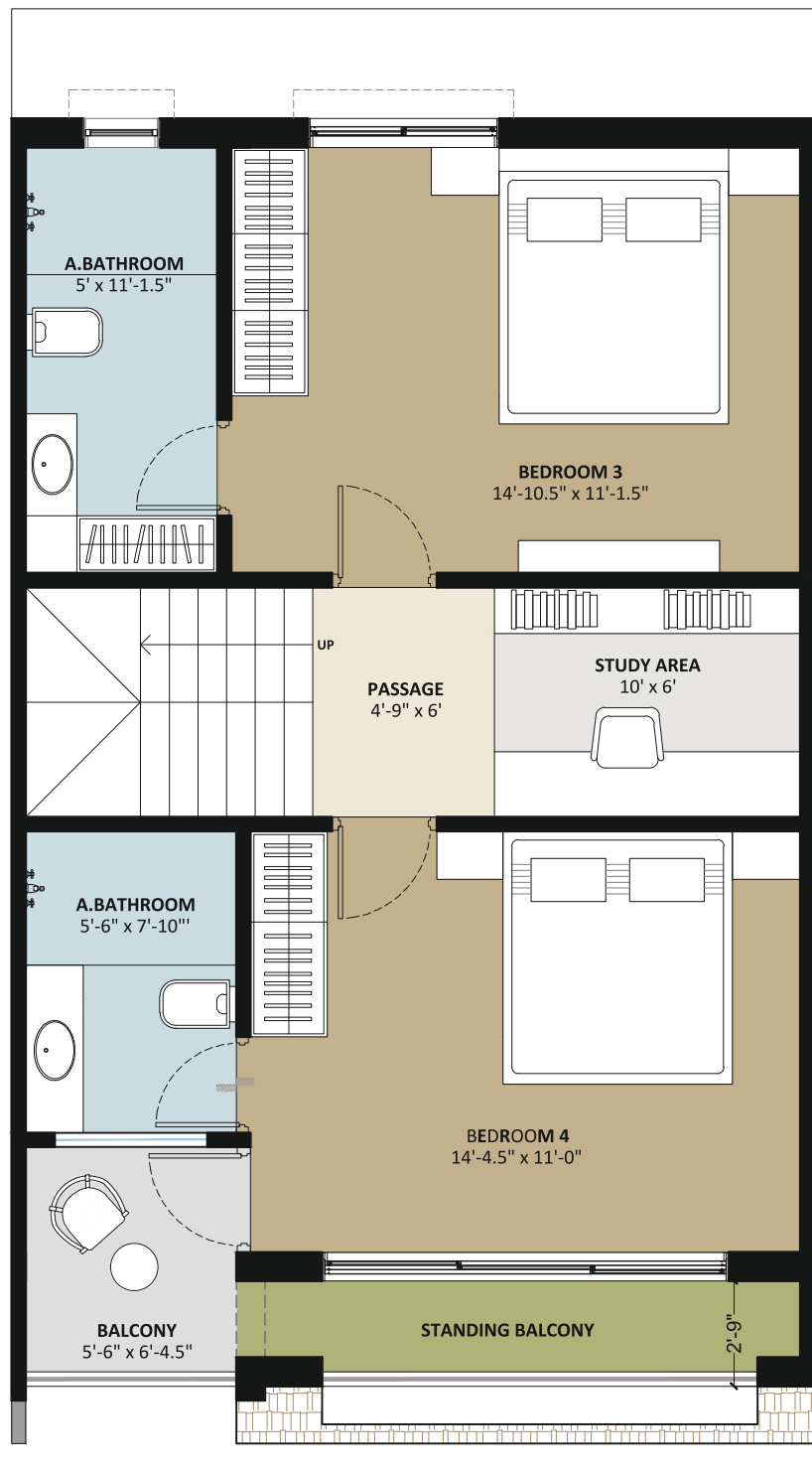
SECOND FLOOR PLAN PLOT SIZE : 21'-0" X 36'-0"
