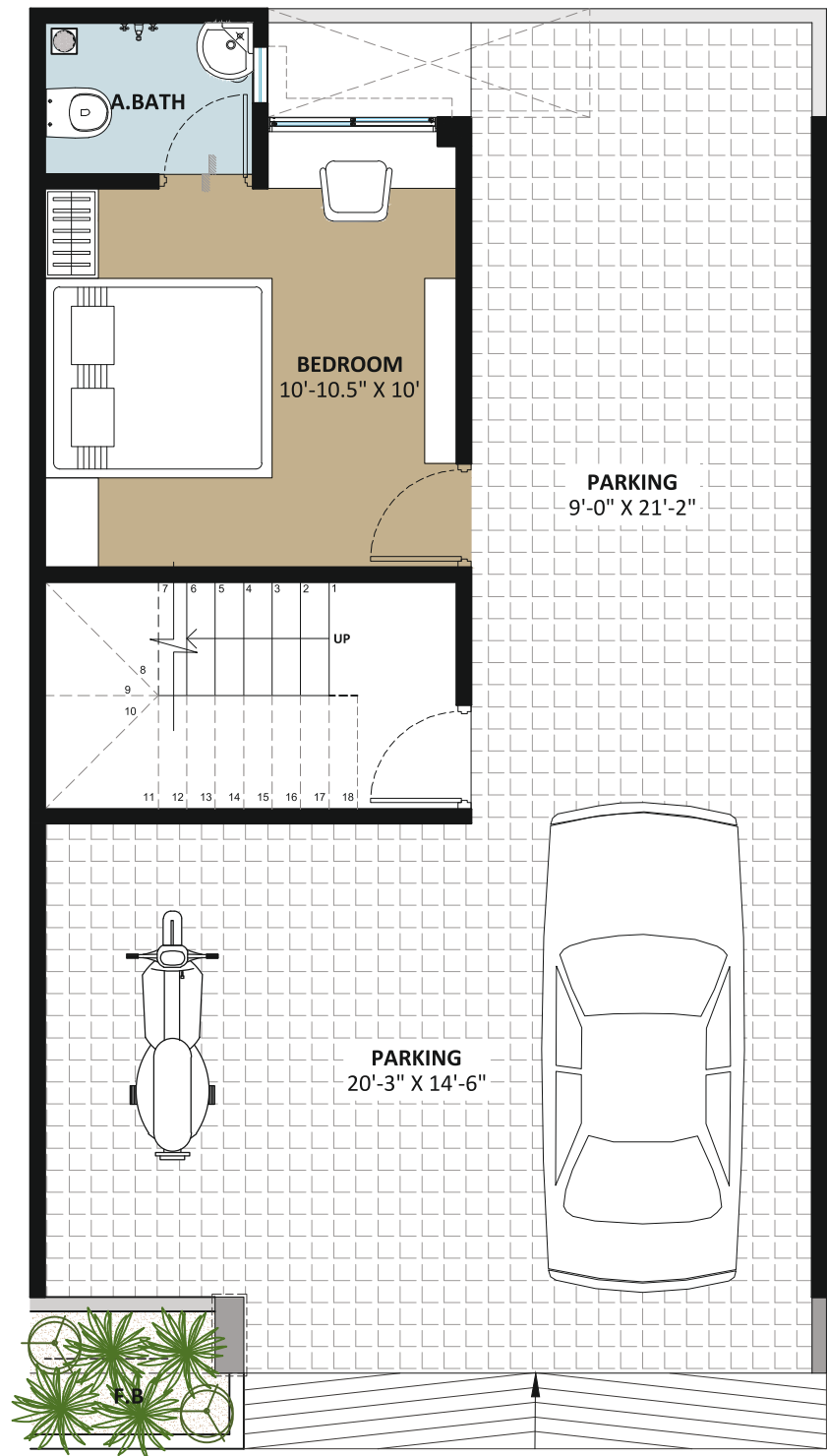
GROUND FLOOR PLAN PLOT SIZE : 21'-0" X 36'-0"
